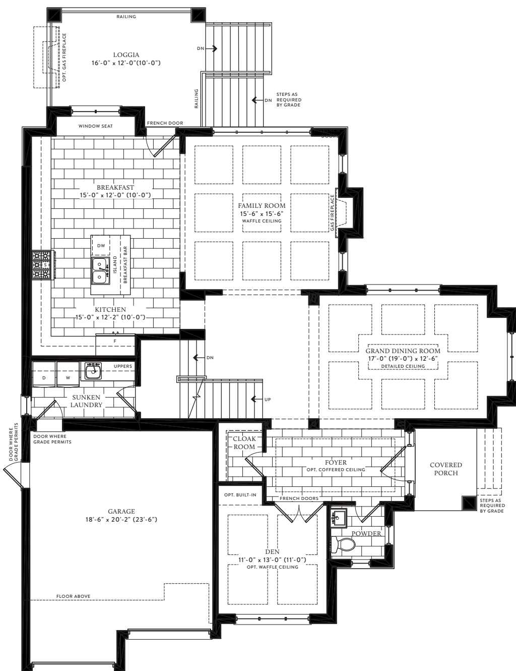
FIRST FLOOR
