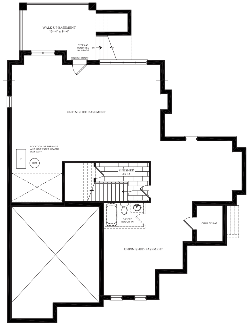
BASEMENT
