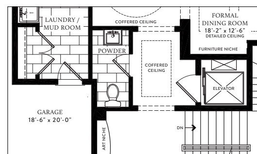
PARTIAL FIRST FLOOR WITH OPT. ELEVATOR
